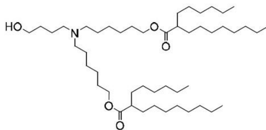
ALC-0315
